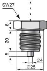
G1/2 type M type G1/2", Ø4 hole M20×1.5, Ø4 hole
